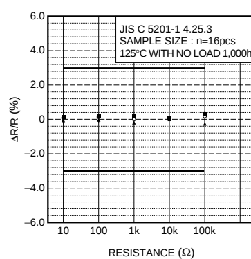
Fig.9 Endurance
