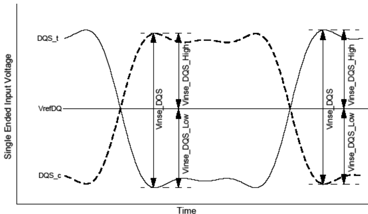
DQS Single-Ended Input Voltage
