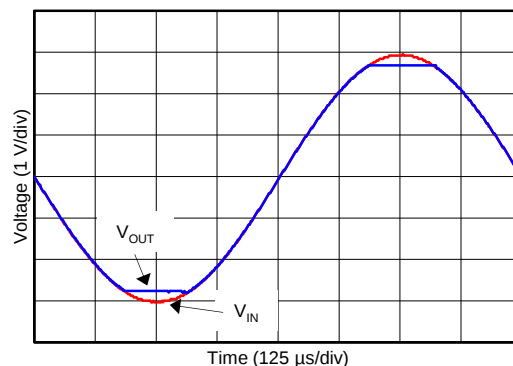
Figure 28. 无相位反转
