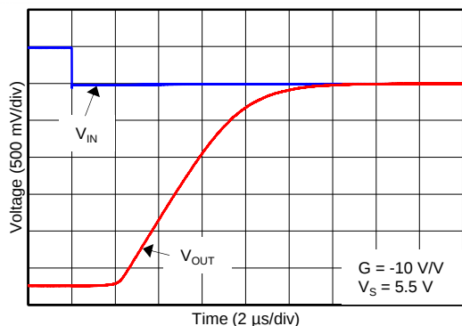
Figure 27. 负过载恢复
