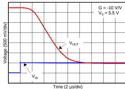
Figure 26. 正过载恢复
