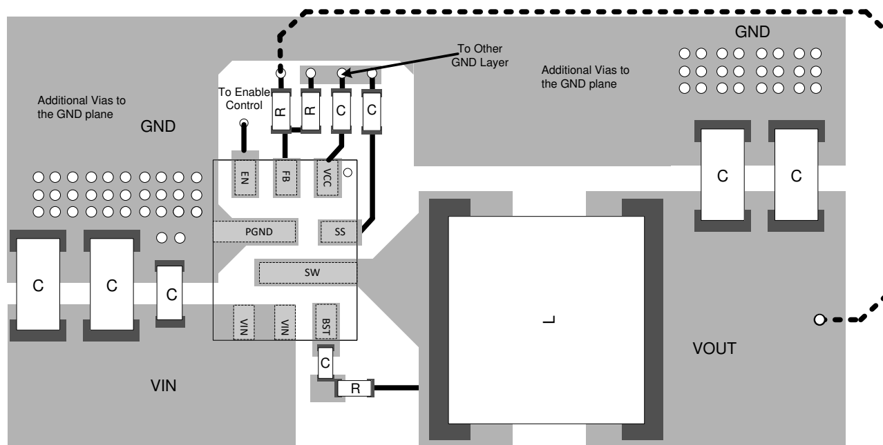
图 7-26. Top-Layer Layout
