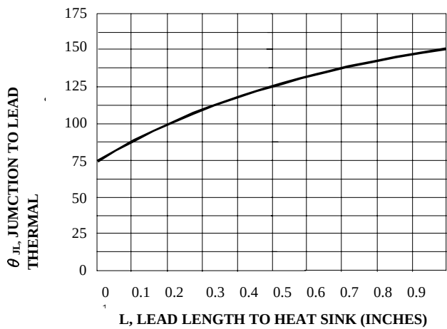
Figure 3. Typical Thermal Resistance versus Lead
