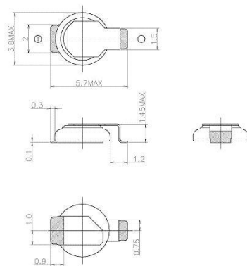
311-VA6R type
