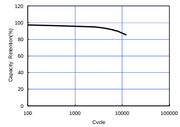
Cycle characteristics
