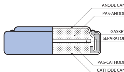
Coin type
