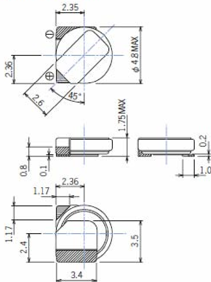
414-VG1 type
