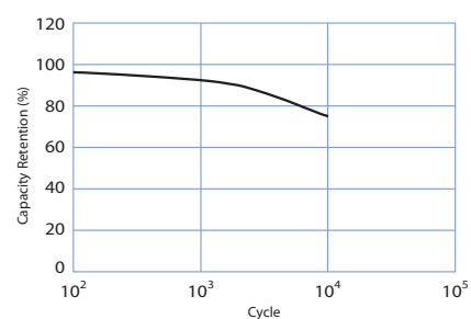
Cycle characteristics
