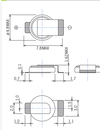
414-VA5R type
