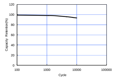
Cycle characteristics
