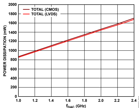
Figure 60. Total Power Dissipation vs. f_{DAC} , 4-Channel DOCSIS, f_{OUT} = 915 MHz, Full-Scale Current = 25 mA (Datapath Configuration: QAM Encoder On, SRRC Filter On, Four 2× Interpolation Filters On)
