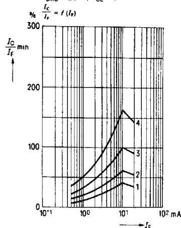
Minimum current transfer ratio versus diode forward current T_{amb} = 25^\circ\text{C} , V_{CE} = 5 V
