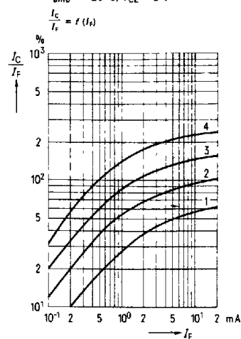
Current transfer ratio (typ.) versus diode forward current T_{amb} = -25^\circ\text{C} , V_{CE} = 5 V
