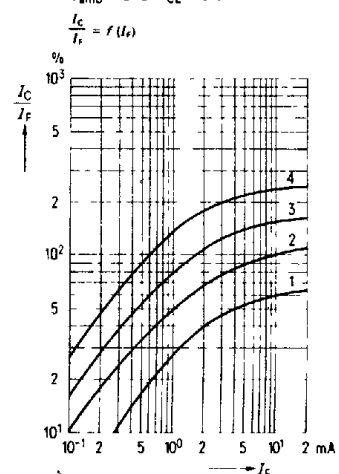
Current transfer ratio (typ.) versus diode forward current T_{amb} = 0^\circ\text{C} , V_{CE} = 5 V
