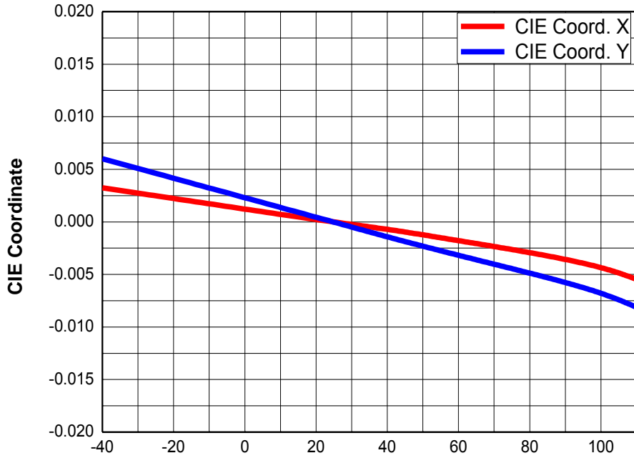
Fig 8. Chromaticity Coordinate vs. Junction Temperature, I_f = 10\text{mA}
