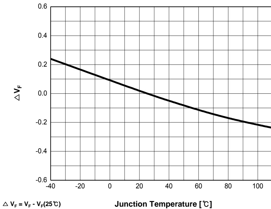
Fig 7. Junction Temperature vs. Forward Voltage Shift, I_F = 10\text{mA}
