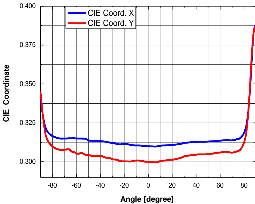
Fig 10. Color. vs. Viewing Angle, T_j = 25^\circ\text{C} , I_F=10\text{mA}
