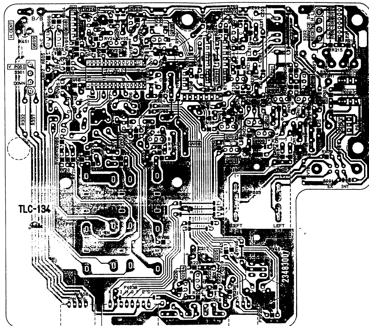
BACK TERMINAL BOARD PB0987 BOTTOM (FOIL) SIDE
