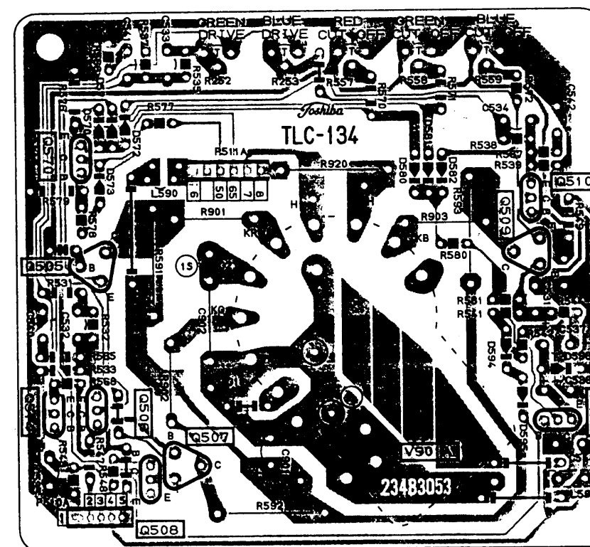
CRT DRIVE BOARD PB0986-1 BOTTOM (FOIL) SIDE
