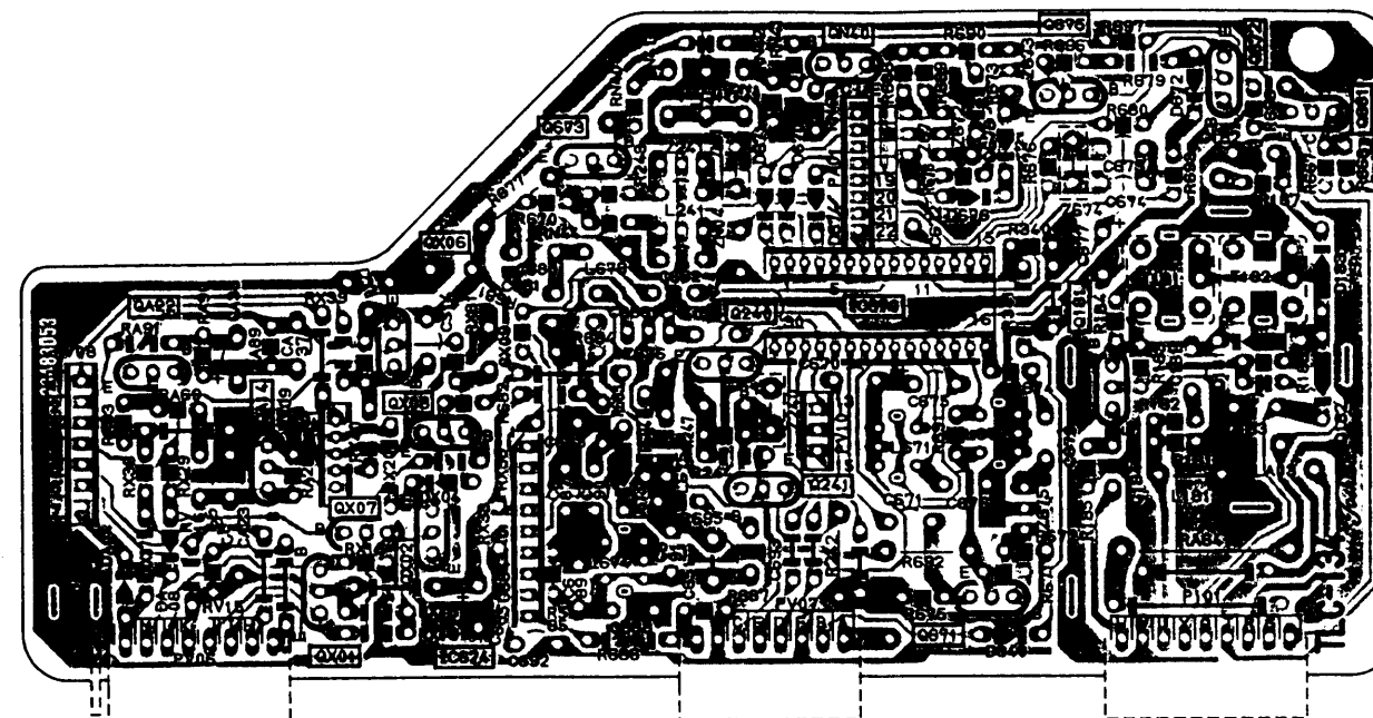
SYSTEM BOARD PB0986-4 BOTTOM (FOIL) SIDE
