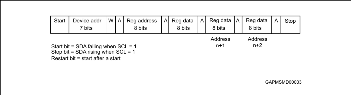
Figure 16. Write operation
