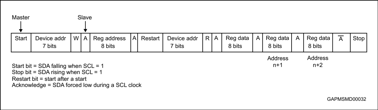
Figure 15. Read operation
