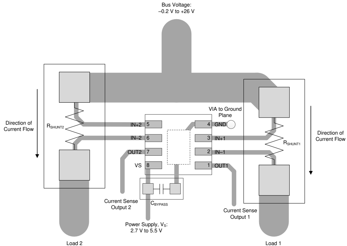
Figure 53. Dual-Channel Recommended Layout (WSN)
