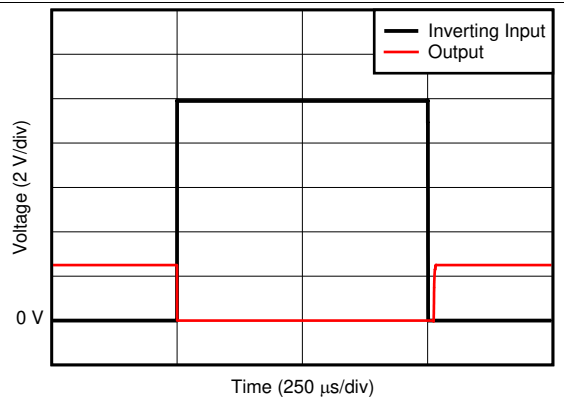
Figure 31. Step Response
