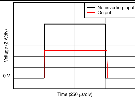
Figure 32. Common-Mode Voltage Transient Response
