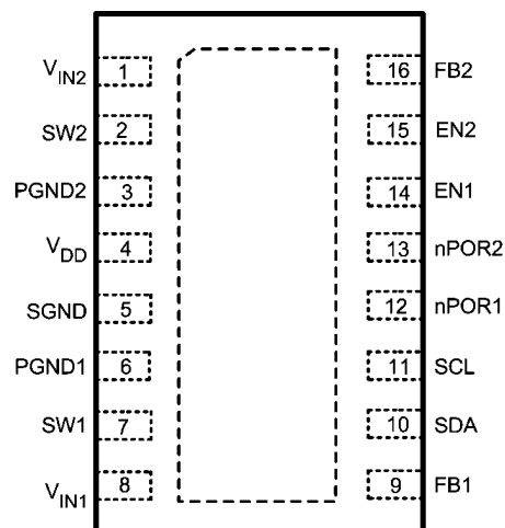
FIGURE 4. Top View
