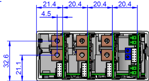
Figure 7 - Rear View
