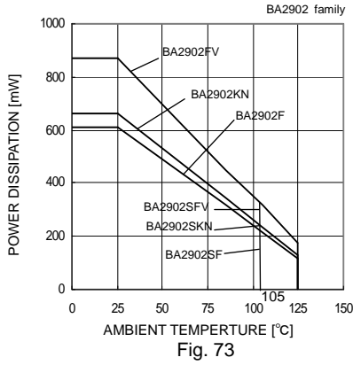
Fig. 73 Derating Curve
