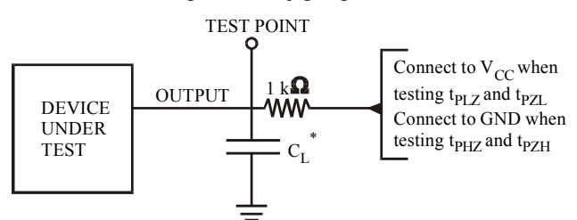
Figure 6. Test Circuit
