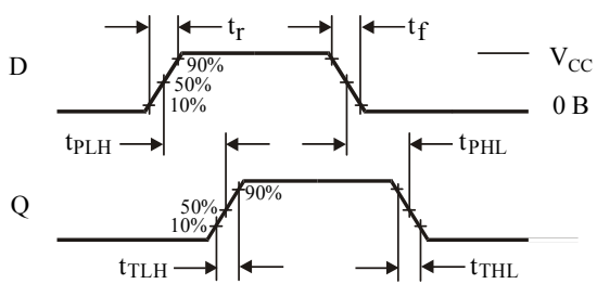
Figure 1. Switching Waveforms
