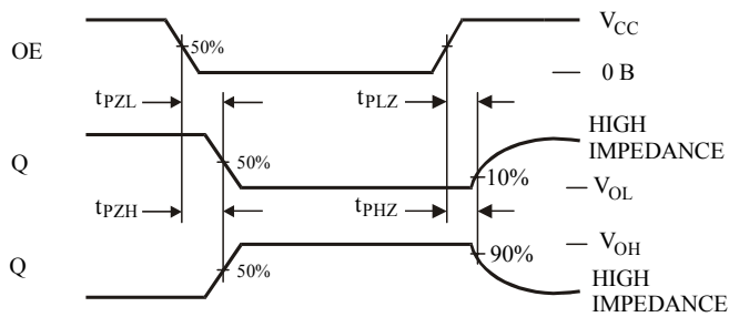
Figure 3. Switching Waveforms
