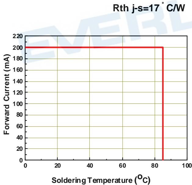
Fig.5 – Max. Driving Forward Current vs. Soldering Temperature
