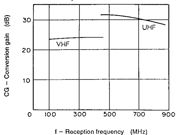
Conversion Gain vs. Reception Frequency (Untuned Input) Input level is -40\text{dBm}
