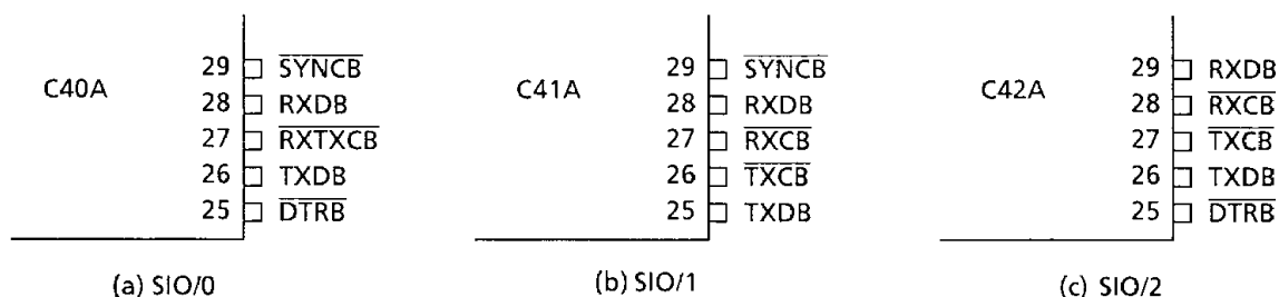
Figure 2.2 (a) SIOs Version (40-pin DIP, 40-pin SOP)
