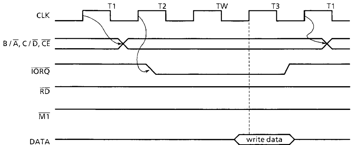
Figure 3.7 Write Timing
