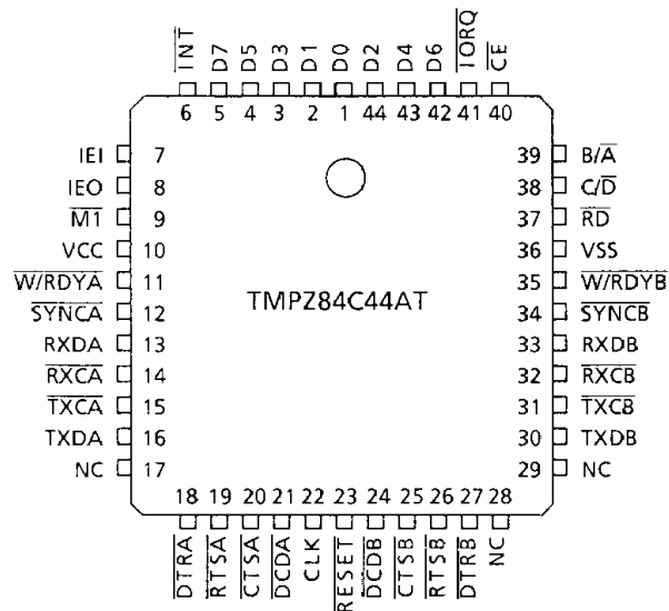
Figure 2.5 Pin Connections of TMPZ84C44A (Top View)
