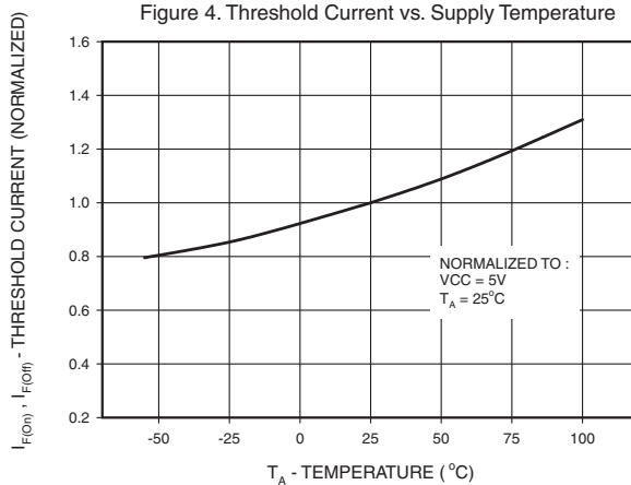
Figure 4. Threshold Current vs. Supply Temperature
