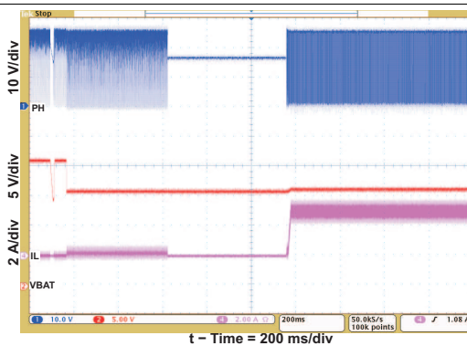
Figure 7. 100% Duty and Refresh Pulse
