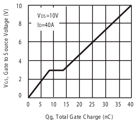
Figure 9. Gate Charge
