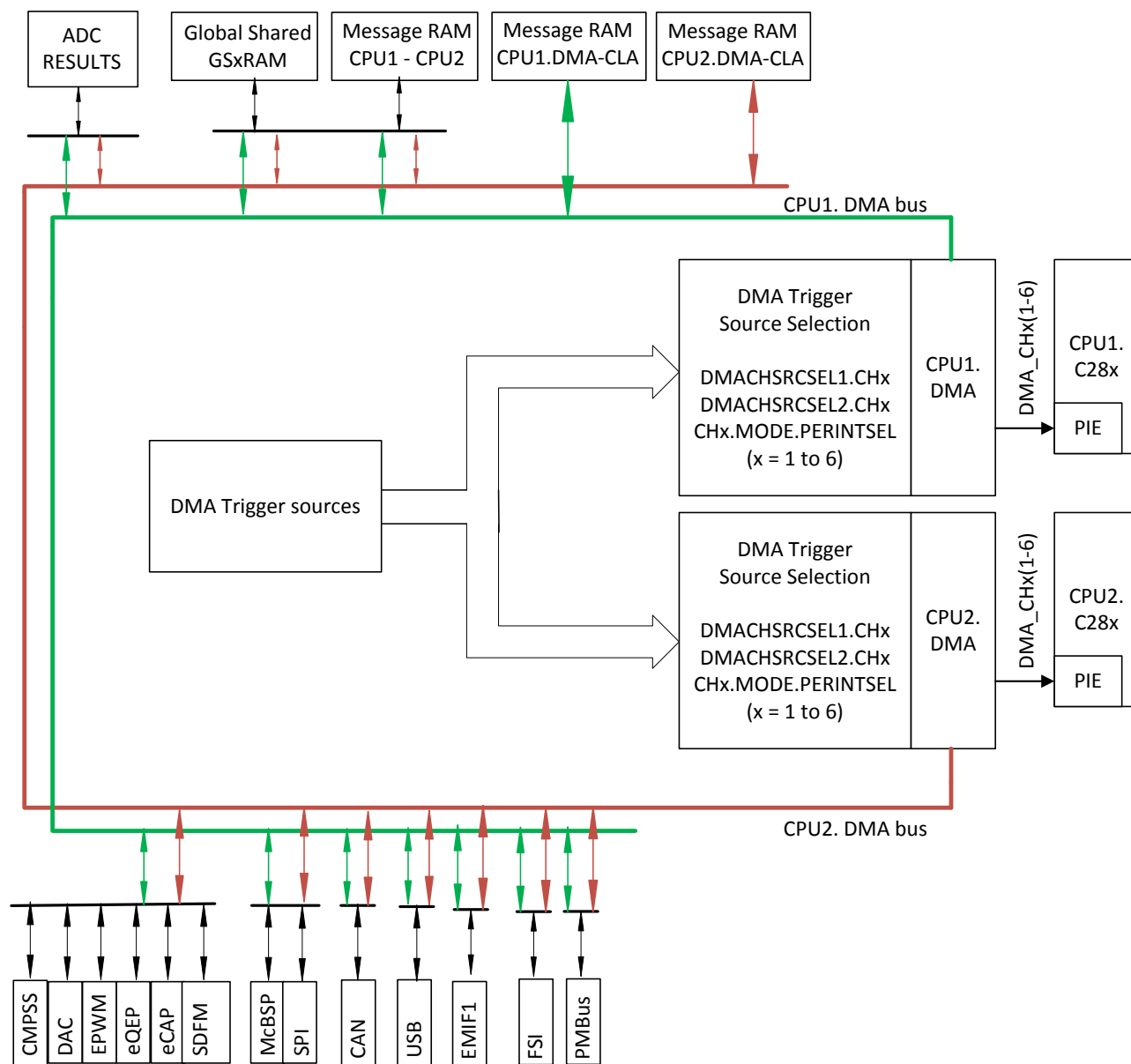
图 8-5. DMA Block Diagram
