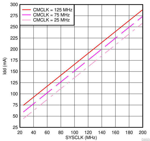
图 7-3. Typical Operating Current Versus SYSCLK
