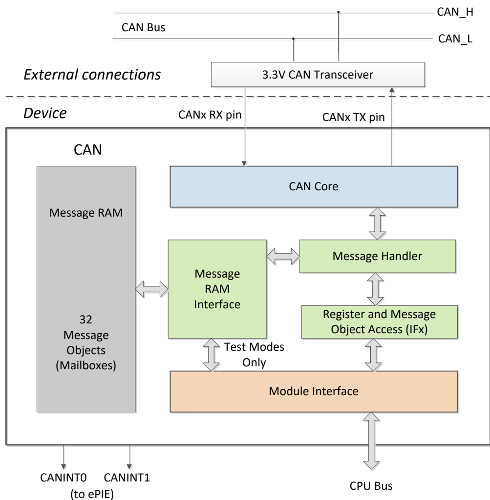
图 7-58. CAN Block Diagram
