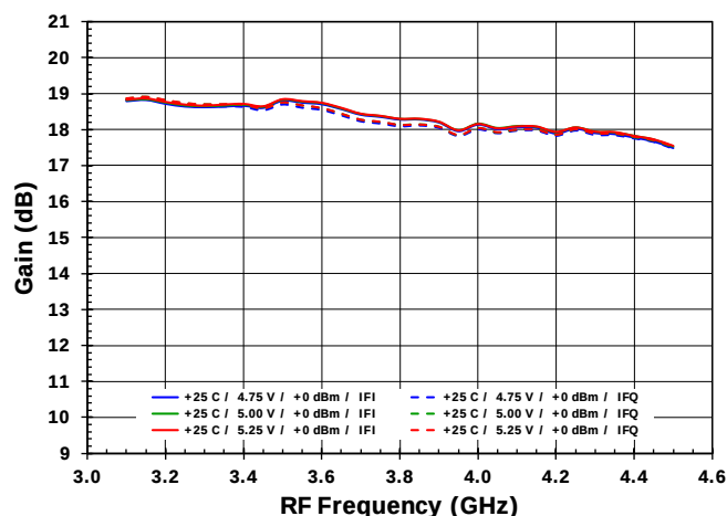
Figure 6. Gain vs. V_{cc} [Low Side LO, RF_Y ]
