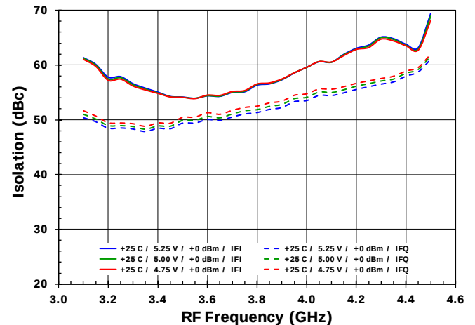
Figure 62. RF_Y to IF Isolation vs. V_{cc} [Low Side LO]
