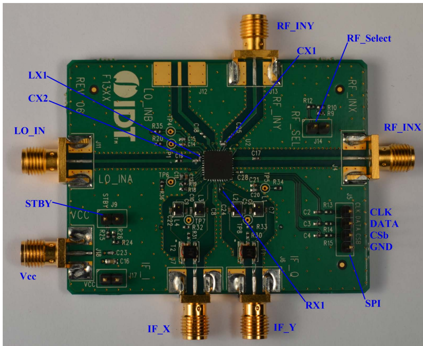
Figure 120. Top View
