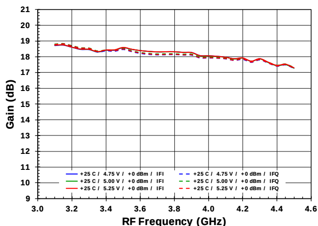
Figure 5. Gain vs. V_{cc} [Low Side LO, RF_X ]
