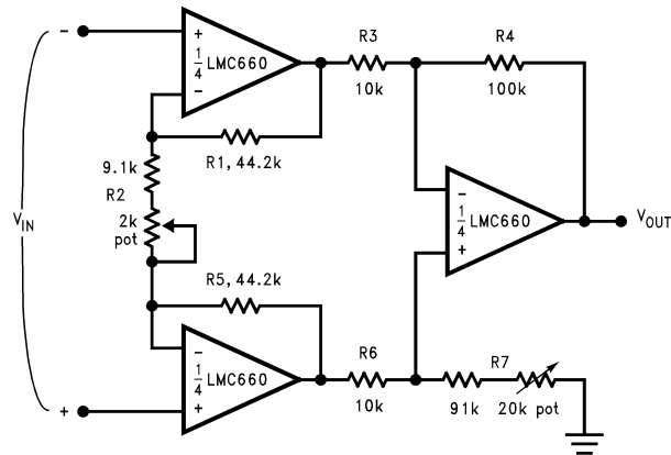
Figure 24. Instrumentation Amplifier
