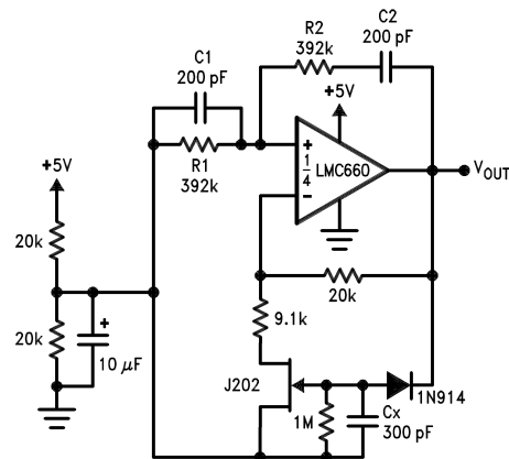
Figure 25. Sine-Wave Oscillator
