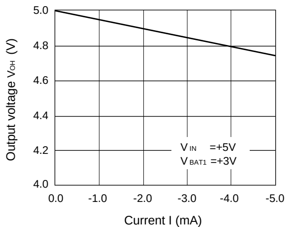
5. V_{OH} characteristics of \overline{ALM} pin
