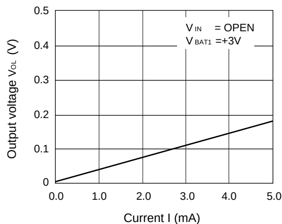
6. V_{OL} characteristics of \overline{ALM} pin
