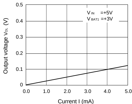
4. V_{OL} characteristics of \overline{RESET} pin
