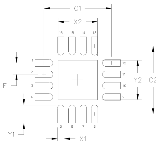
Figure 7.1. 16-Pin QFN Land Pattern
