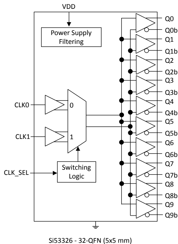
Figure 4.6. Si533326 Block Diagram
