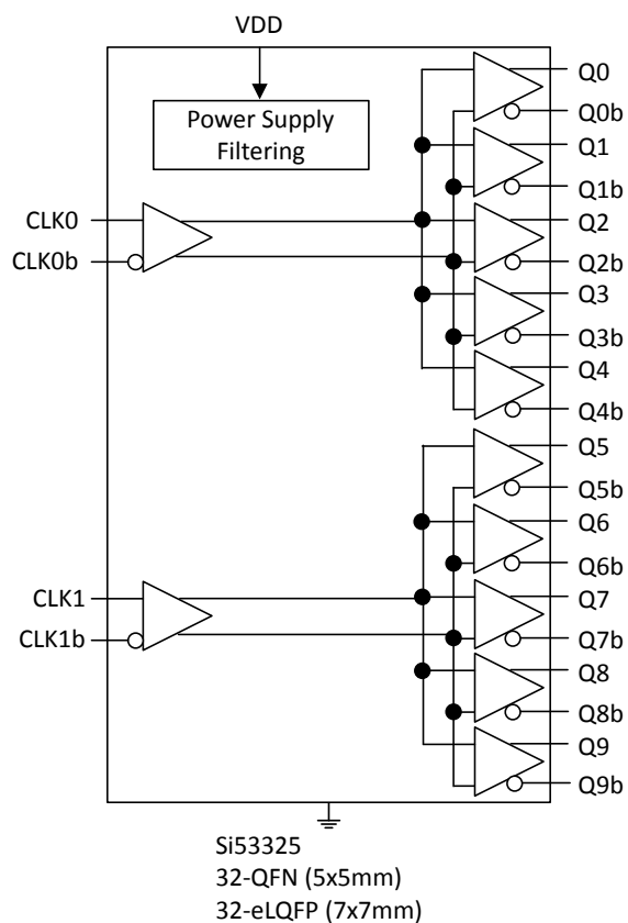
Figure 4.5. Si533325 Block Diagram
