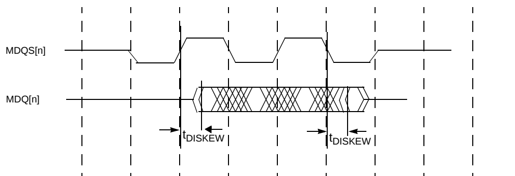
Figure 4. DDR SDRAM Interface Input Timing
