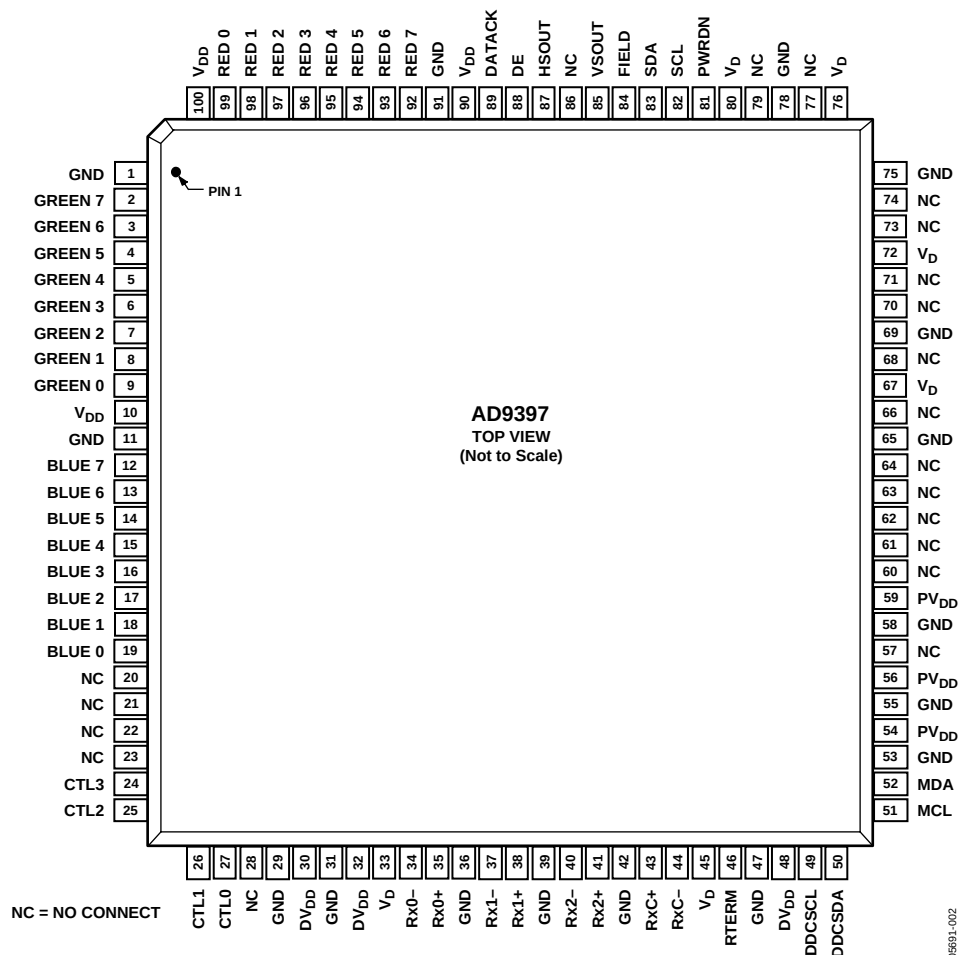
Figure 2. Pin Configuration
