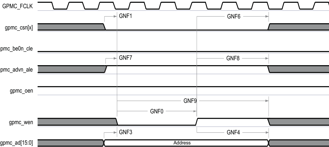
Figure 5-24. GPMC/NAND Flash—Address Latch Cycle
