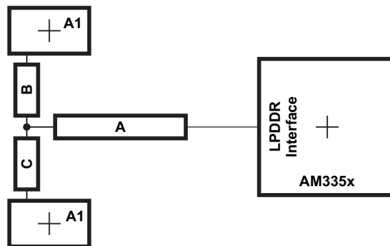
Figure 5-31. CK and ADDR_CTRL Routing and Topology
