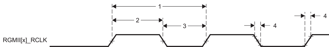
Figure 5-8. RGMII[x]_RCLK Timing - RGMII Mode
