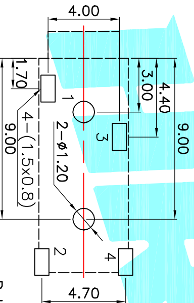
P.C.B LAYOUT(copper-sided view)
