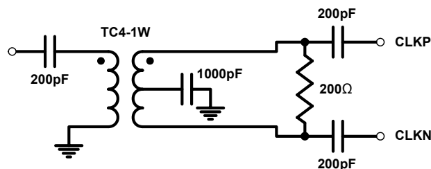
FIGURE 29. RECOMMENDED CLOCK DRIVE
