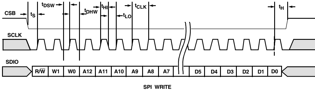
FIGURE 35. SPI WRITE
