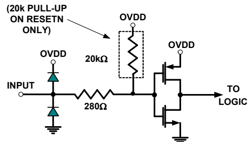
FIGURE 44. DIGITAL INPUTS
