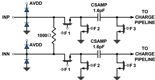
FIGURE 41. ANALOG INPUTS
