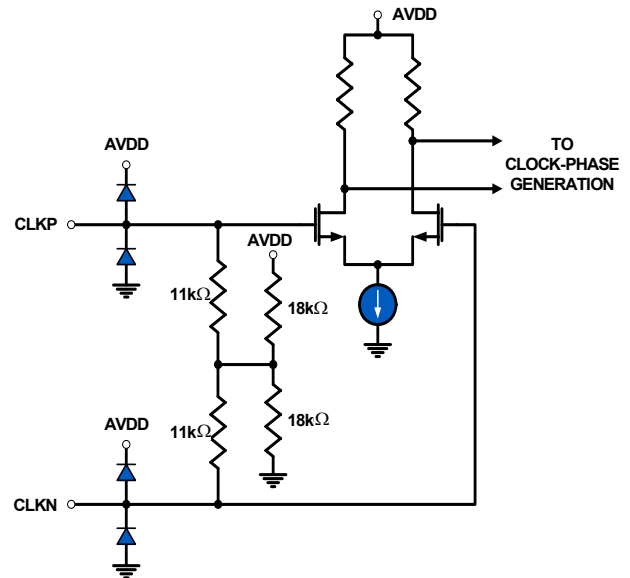
FIGURE 42. CLOCK INPUTS
