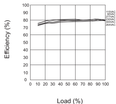
RAC04C-12SH
