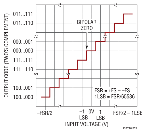
Figure 2. LTC2377-16 Transfer Function
