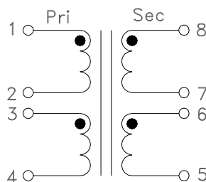
Schematic A
