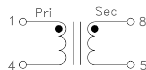
Schematic B
