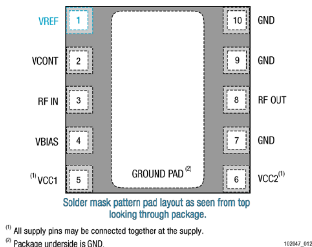
Figure 10. Pin Names and Configuration (Top View)
