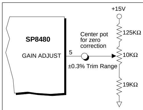
Figure 2. Gain Adjust
