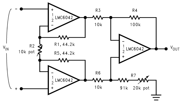
FIGURE 10. Instrumentation Amplifier
