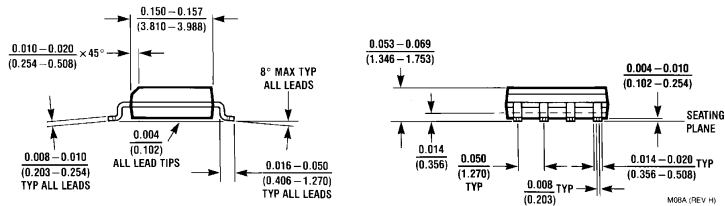
8-Pin Small Outline Package Order Number LMC6042AIM or LMC6042IM NS Package Number M08A
