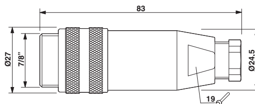
Dimensional drawing
