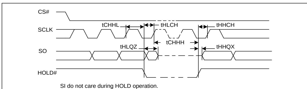
Figure50. Hold Timing
