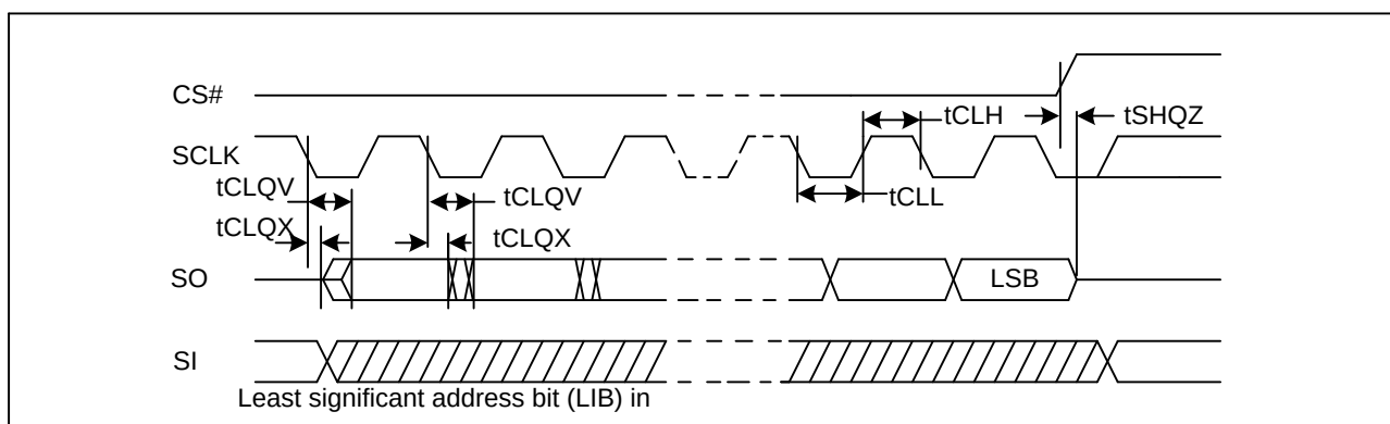
Figure48. Output Timing
