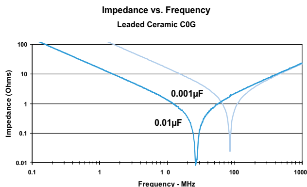
Figure 10. Impedance vs Frequency for C0G Dielectric
