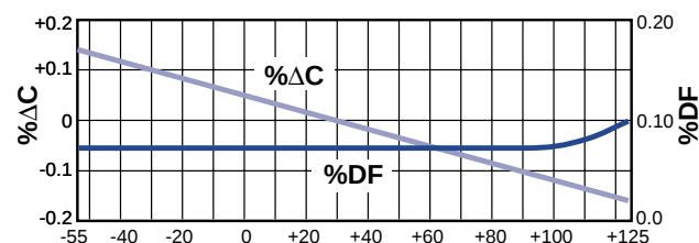
Figure 3. Temperature °C Capacitance & DF vs Temperature - C0G
