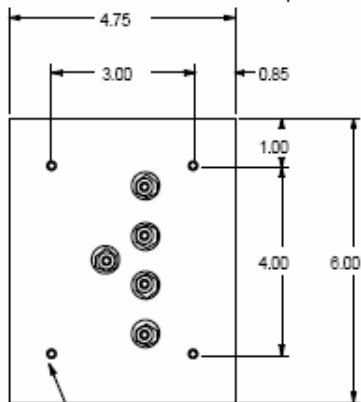
1/4-20 UNC MOUNTING STUD (8 PL)
