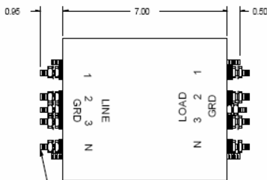
1/4-20UNC THD. TERMINAL (10 PL) (.75 DIA BUSHING)
