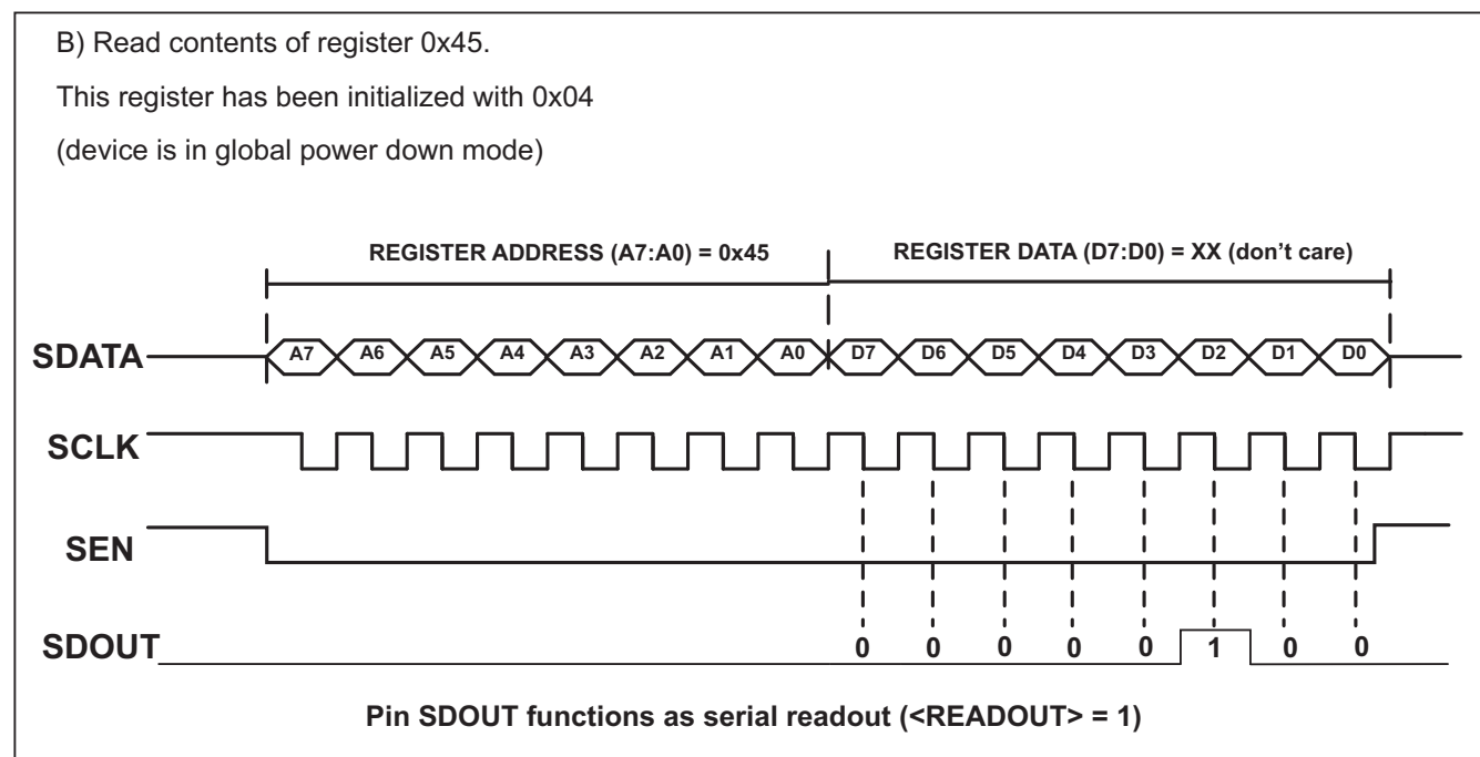
Figure 7. Serial Readout
