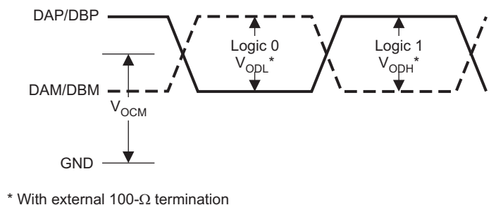
Figure 2. LVDS Output Voltage Levels
