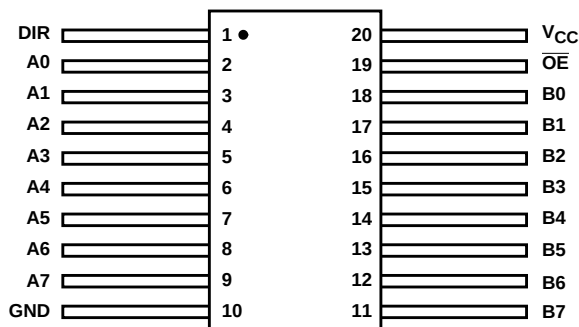
HCTS245KTR (FLATPACK), CDIP4-F20 TOP VIEW
