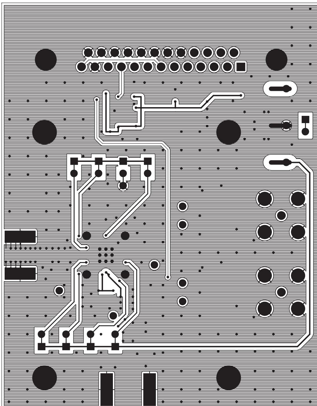
Figure 4. MAX2112 EV Kit PCB Layout—Bottom
