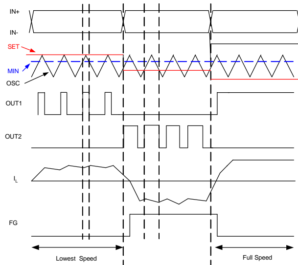
Figure 1. Rotation Waveform
