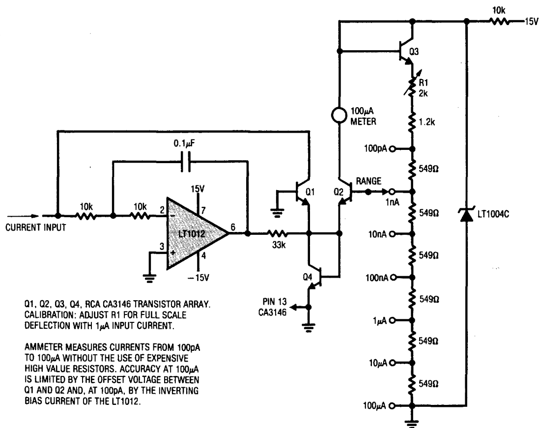
Ammeter with Six Decade Range
