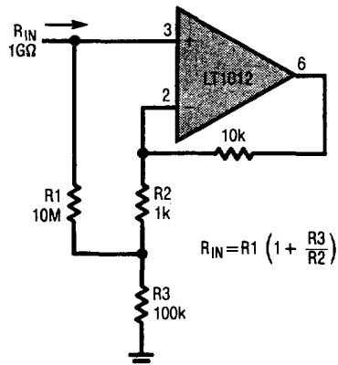
Resistor Multiplier
