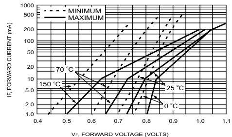
FIG.2- TYPICAL FORWARD CHARACTERISTICS
