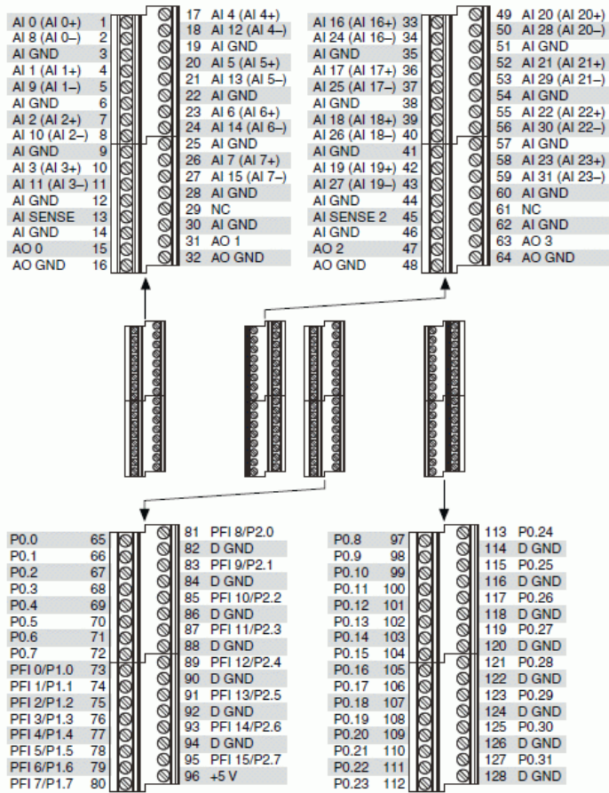
NI USB-6343 Pinout
