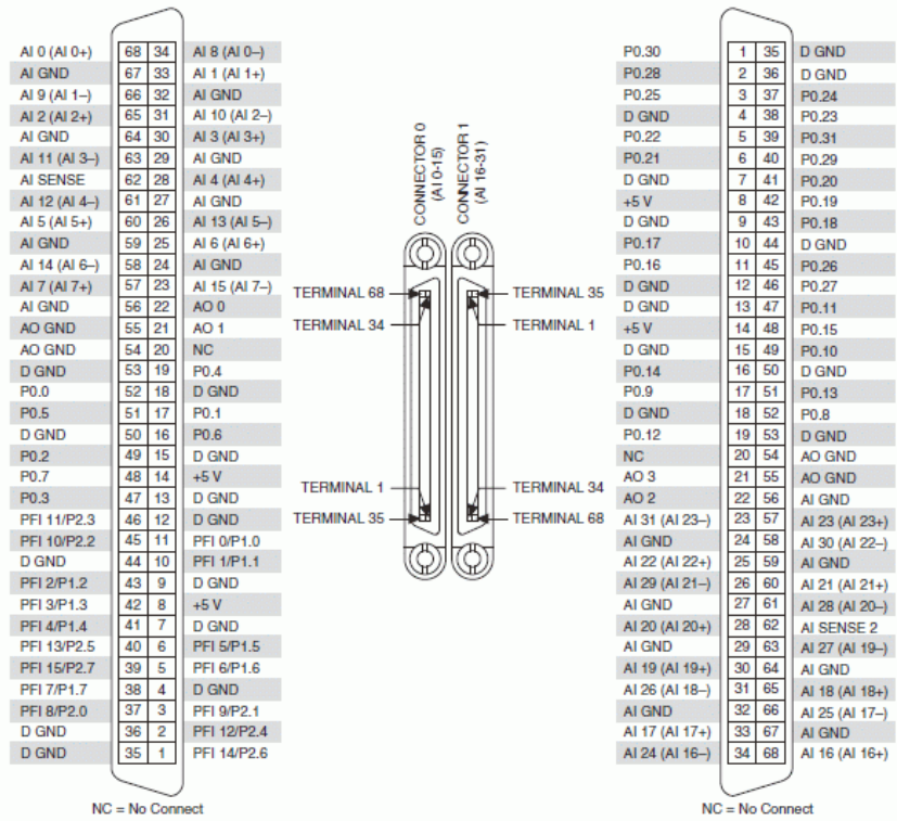
NI PCIe-6343 Pinout
