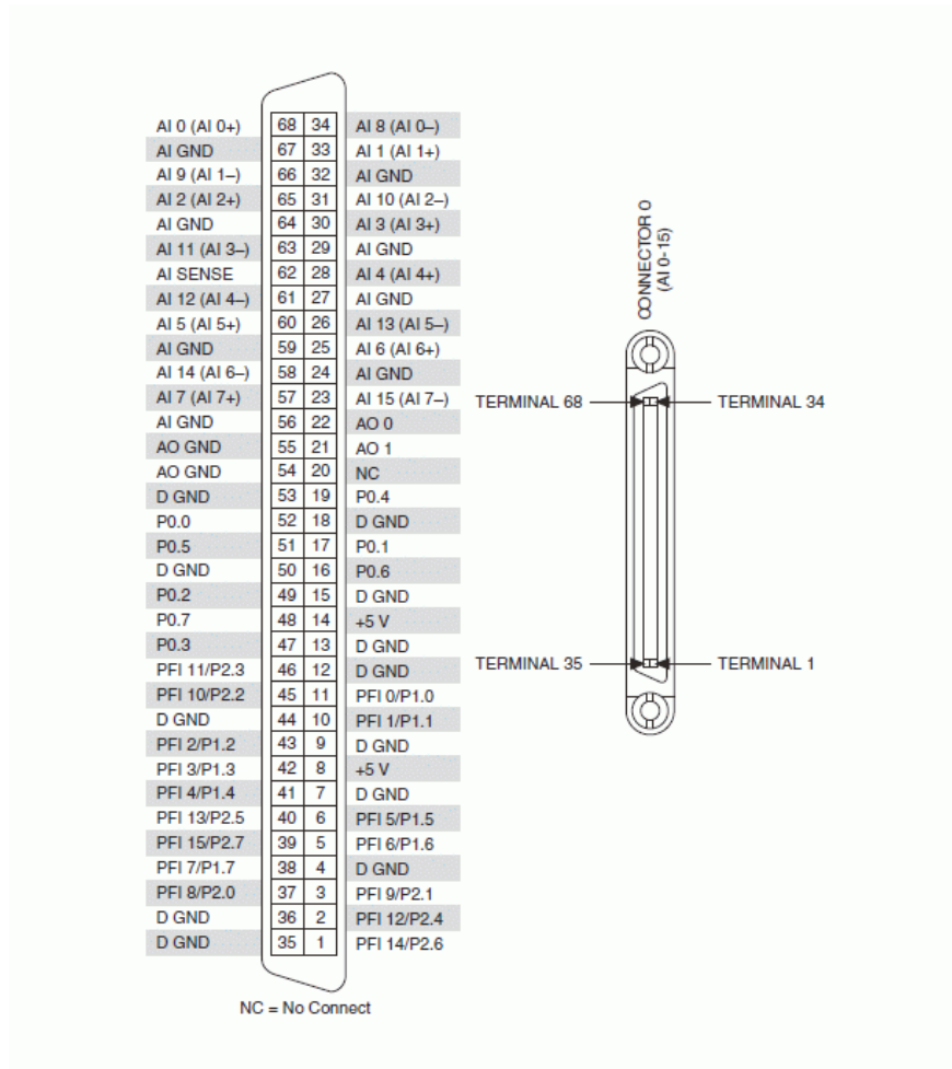
NI PCIe/PXle-6341 Pinout
