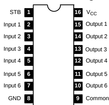
Pin Connection Diagram
